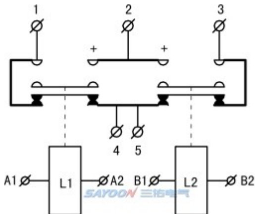
Paired Single Pole Double Throw Contactor. 1.2.3.4.5 Contact Terminal A1.A2.B1.B2 for the two sets of coil terminal
